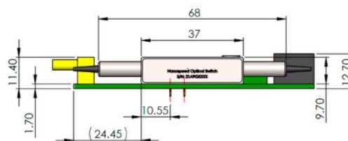
Driver with Package A
